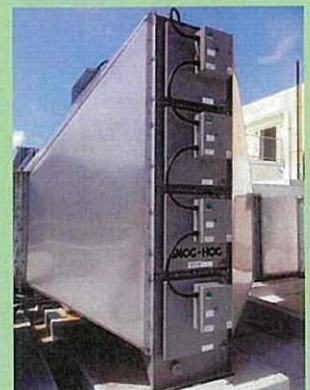
SMOG-HOG Electrostatic Precipitator installed at Kee Wah Factory 奇華工廠內的靜電除油煙器
